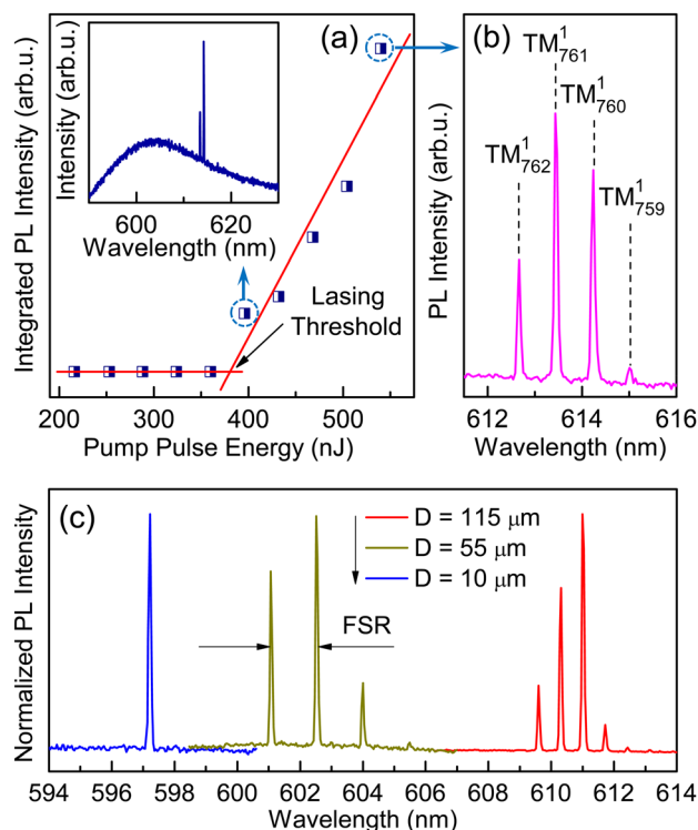
FIG. 3. (a) Evaluation of lasing threshold from hemisphere with D \sim 104 \mu\text{m} . The inset demonstrates a spectrum just above lasing threshold. (b) Lasing mode determination based on WGM theory. (c) Lasing spectra of hemispheres with different diameters.
