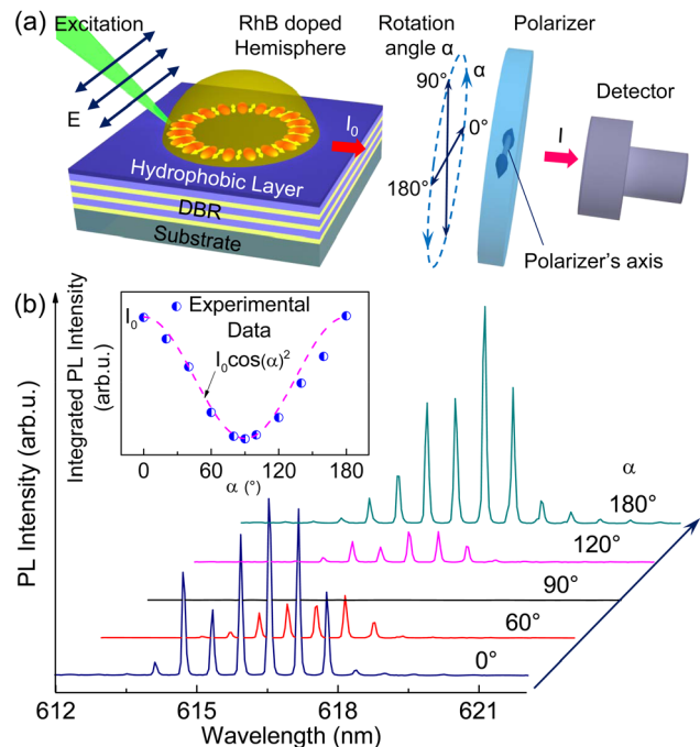
FIG. 2. (a) Schematic diagram of the optical measurement setup. Electric field oscillation ( E ) of the excitation laser is fixed during the experiment. It is parallel to the axis of polarizer at an initial measurement ( \alpha = 0^{\circ} ). The arrows inside the hemisphere indicate electric field oscillation of WGMs (red patterns). (b) The lasing spectra as a function of rotation angle of polarizer \alpha . The inset presents a dependence of integrated lasing intensity with \alpha .
