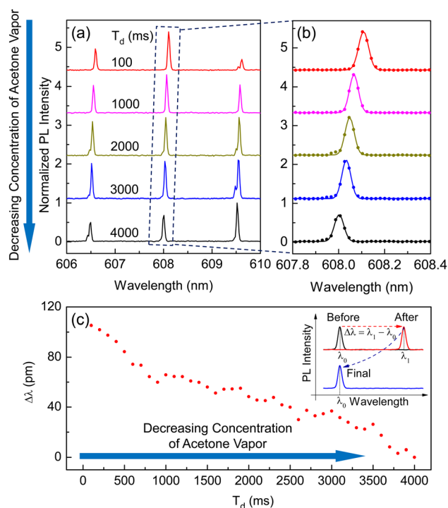
FIG. 4. (a) Lasing spectra from the hemisphere versus diffusion times of acetone vapor ( T_d ) and (b) close-up image of the spectra near 608 nm. The linewidth of lasing mode is around 0.06 nm, corresponding to Q \sim 1 \times 10^4 . (c) Dynamic shift of lasing mode monitoring near 608 nm with T_d . The inset schematically illuminates resonant mode and its position at the time: "Before"—before the sensing vapor is added (black), "After"—after the vapor is added (red), and "Final"—the vapor is completed diffused (blue).
