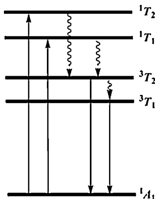
Fig. 5. Schematic model for absorption and emission processes of \text{VO}_4 tetrahedron in \text{Zn}_2\text{V}_2\text{O}_7 .
