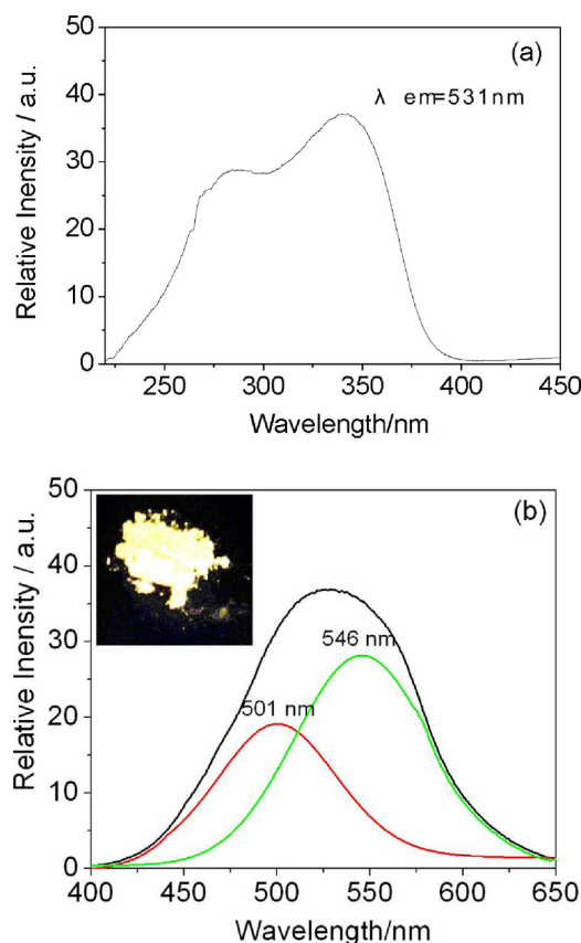
Fig. 3. Photoluminescence spectra of \text{Zn}_2\text{V}_2\text{O}_7 : (a) excitation spectra ( \lambda_{em} = 531 nm); (b) emission spectra ( \lambda_{ex} = 340 nm). Inset: the photograph of \text{Zn}_2\text{V}_2\text{O}_7 under ultraviolet light irradiation.
