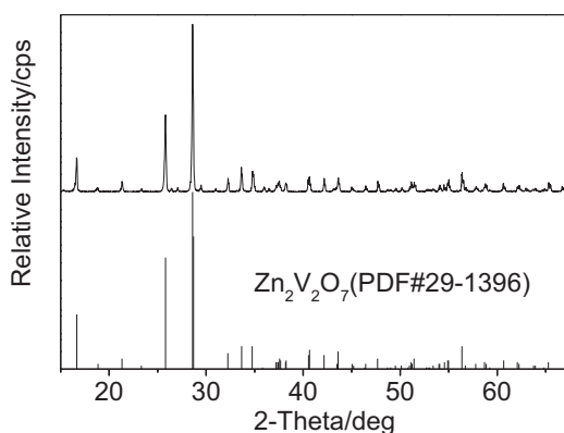
Fig. 1. XRD patterns of \text{Zn}_2\text{V}_2\text{O}_7 prepared at 600 °C.
