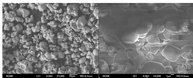
Fig. 2. SEM images of \text{Zn}_2\text{V}_2\text{O}_7 sintered at a 600 °C.
