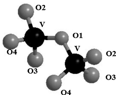
Fig. 4. Vanadium-oxygen (pyro) units in \text{Zn}_2\text{V}_2\text{O}_7 .
