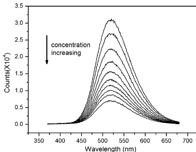
Fig. 4. Fluorescence emission spectra of the dansyl-functionalized film in the presence of nitrobenzene at different concentrations ( \lambda_{\text{ex}} = 350 \text{ nm} ).
