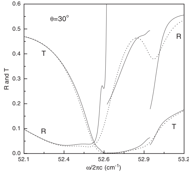
Figure 4. Reflection and transmission versus frequency for an angle of incidence of 30^\circ in such a geometry where the dielectric with \varepsilon = 2.3 is above the film and the space below is a vacuum. The intensity of incident radiation S_1 = 4.7 \text{ kW cm}^{-2} and the dotted lines show the linear results.
