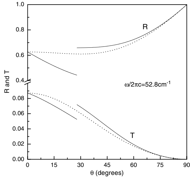
Figure 3. Reflectivity and transmissivity versus angle of incidence for the frequency fixed at 52.8 \text{ cm}^{-1} and the intensity of incident radiation S_I = 4.7 \text{ kW cm}^{-2} . The dotted lines show the linear results.
