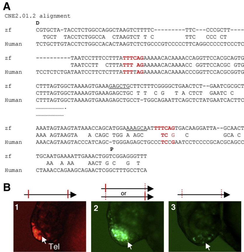
Fig. 5. Mutating the motif TTTCAG impairs the forebrain enhancer activity of CNE2.01.2. (A) Alignment of zebrafish and human CNE 2.01.2. Abbreviations: D, distal to the transcription start site; P, proximal to the transcription start site. (B) Functional validation of de novo predicted motifs in the CNE2.01.2. Reporter activity of (1) The CNE containing the wildtype copies of the motif TTTCAG, or mutations in the following motif: (2) either the distal or the proximal copy of the motif; (3) Mutating both copies of the motif.
