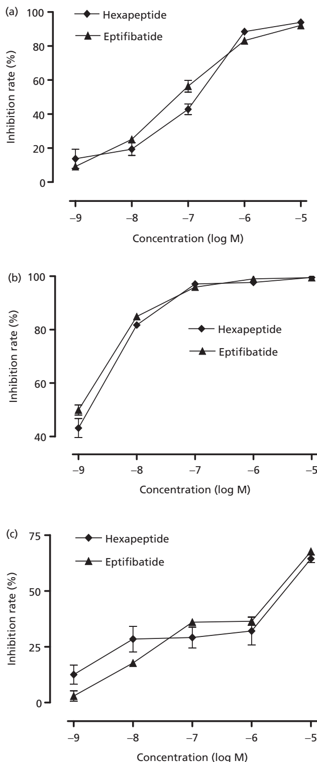
Figure 1 The concentration–inhibition curves of hexapeptide on dog platelet aggregation induced by 50 \mu M adenosine diphosphate (a), 1.0 mM arachidonic acid (b) and 0.4 U/ml thrombin (c). Data are means \pm SEM, n = 6 . * P < 0.05 and ** P < 0.01 vs control.
