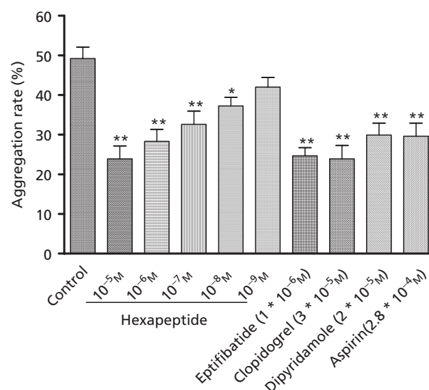
Figure 2 Inhibitory effect of hexapeptide on rat platelet aggregation induced by 50 \mu M adenosine diphosphate. Data are means \pm SEM, n = 6 . * P < 0.05 and ** P < 0.01 vs control.
