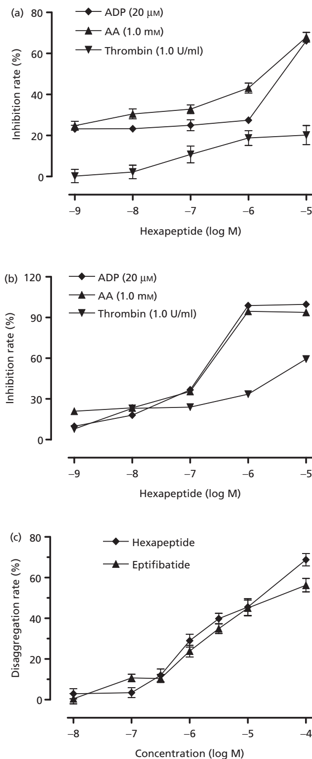
Figure 4 The concentration-inhibition curves of hexapeptide on rabbit platelet aggregation induced by 20 \mu M adenosine diphosphate (ADP), 1.0 mM arachidonic acid (AA) and 1.0 U/ml thrombin (a). The concentration-inhibition curves of hexapeptide on human platelet aggregation induced by 20 \mu M ADP, 1.0 mM AA and 1.0 U/ml thrombin (b). Disaggregation effects of hexapeptide and eptifibatide on dog platelets induced by 50 \mu M ADP (c). Data are means \pm SEM, n = 6 .
