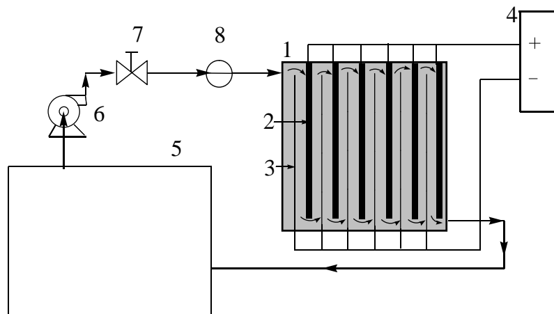
Figure 1. Schematic diagram of the experimental setup. (1) electrochemical cell; (2) anodes; (3) cathodes; (4) controlled DC unit; (5) reservoir; (6) pump; (7) flow regulator; (8) flow meter
