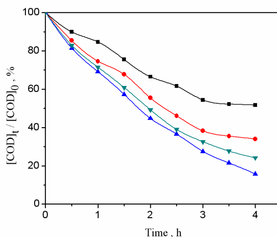
Figure 3. Effect of the initial pH on the variation of [\text{COD}]_t/[\text{COD}]_0 with electrolysis time. (■) pH 6; (●) pH 8; (▼) pH 11; (▲) pH 13. [\text{CN}^-]_0 = 250 \text{ mg/L} ; applied current density = 30 \text{ mA cm}^{-2} ; flow rate = 80 \text{ L/h} .
