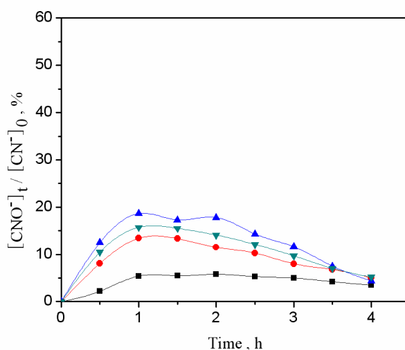
Figure 4. Effect of the initial pH on the variation of [\text{CNO}^-]_t/[\text{CN}^-]_0 with electrolysis time. (■) pH 6; (●) pH 8; (▼) pH 11; (▲) pH 13. [\text{CN}^-]_0 = 250 \text{ mg/L} ; applied current density = 30 \text{ mA cm}^{-2} ; flow rate = 80 \text{ L/h} .
