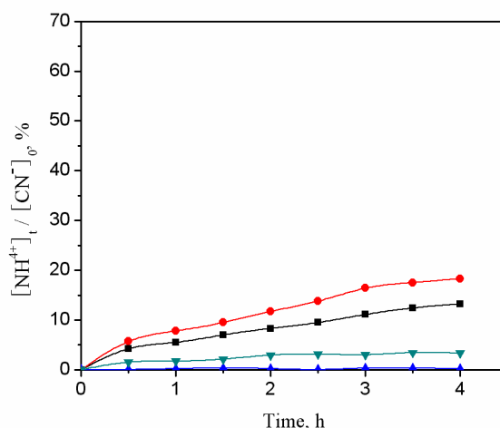
Figure 5. Effect of the initial pH on the variation of [\text{NH}_4^+]_t/[\text{CN}^-]_0 with electrolysis time. (■) pH 6; (●) pH 8; (▼) pH 11; (▲) pH 13. [\text{CN}^-]_0 = 250 \text{ mg/L} ; applied current density = 30 \text{ mA cm}^{-2} ; flow rate = 80 \text{ L/h} .
