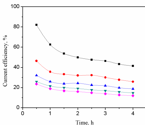
Figure 7. Current efficiency for current densities with electrolysis time at initial pH 13. (■) 10 mA cm -2 ; (●) 20 mA cm -2 ; (▲) 30 mA cm -2 ; (▼) 40 mA cm -2 ; (◆) 50 mA cm -2 . [CN - ] 0 = 250 mg/L; flow rate = 80 L/h.
