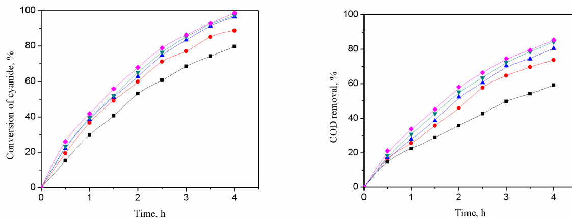
Figure 6. Effect of current density on the conversion of cyanide and COD removal with electrolysis time at initial pH 13. (■) 10 mA cm -2 ; (●) 20 mA cm -2 ; (▲) 30 mA cm -2 ; (▼) 40 mA cm -2 ; (◆) 50 mA cm -2 . [CN - ] 0 = 250 mg/L; flow rate = 80 L/h.
