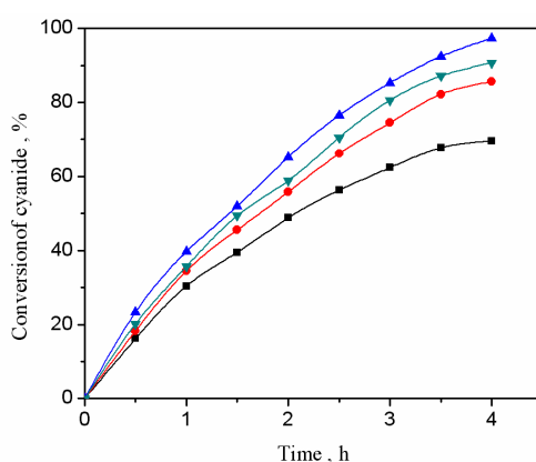
Figure 2. Effect of the initial pH on the conversion of cyanide with electrolysis time. (■) pH 6; (●) pH 8; (▼) pH 13; (▲) pH 13. [\text{CN}^-]_0 = 250 \text{ mg/L} ; applied current density = 30 \text{ mA cm}^{-2} ; flow rate = 80 \text{ L/h} .
