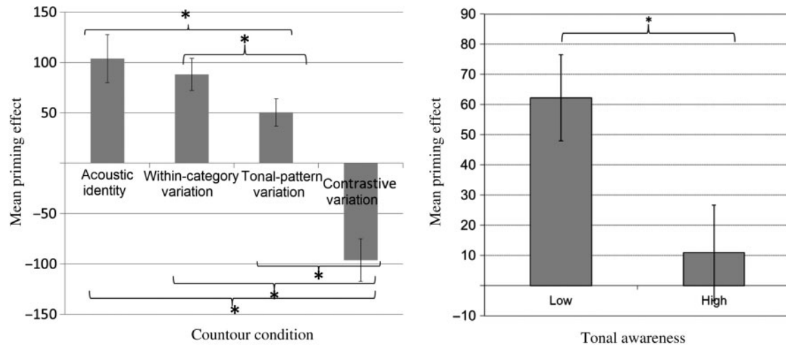
Figure 3. Mean priming effect for each Contour Condition (left) and tonal awareness conditions (right)
