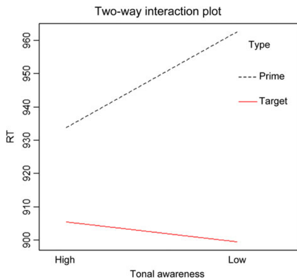
Figure 4. Two-way interaction plot of tonal awareness (high or low) and the type of stimuli (prime or target) on reaction time data
