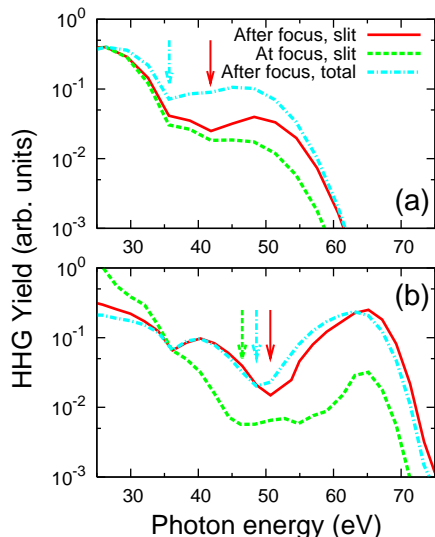
FIG. 6: (Color online) Dependence of macroscopic HHG spectra (envelope only) on experimental arrangements (a) for an 800-nm laser with intensity of 2.1 \times 10^{14} W/cm 2 , and (b) for a 1200-nm laser with intensity of 1.2 \times 10^{14} W/cm 2 . The arrangements are: (1) gas jet after focus and slit is used (solid lines); (2) gas jet at the focus and slit is used (dashed lines); and (3) gas jet is after the focus but without the slit (dot-dashed lines). Arrows indicate the positions of minima. Degree of alignment: \langle \cos^2 \theta \rangle = 0.60 . Pump-probe angle \alpha = 0^\circ .
