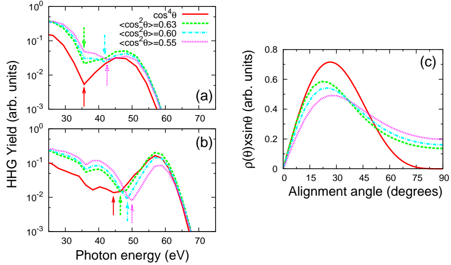
FIG. 4: (Color online) Dependence of macroscopic HHG spectra (envelope only) with degrees of molecular alignment distributions for (a) an 800-nm laser with intensity of 1.8 \times 10^{14} W/cm 2 , and (b) a 1200-nm laser with intensity of 1.0 \times 10^{14} W/cm 2 . The weighted angular distributions of the molecules are shown in (c). Arrows indicate the positions of minima. Pump-probe angle \alpha=0^\circ .
