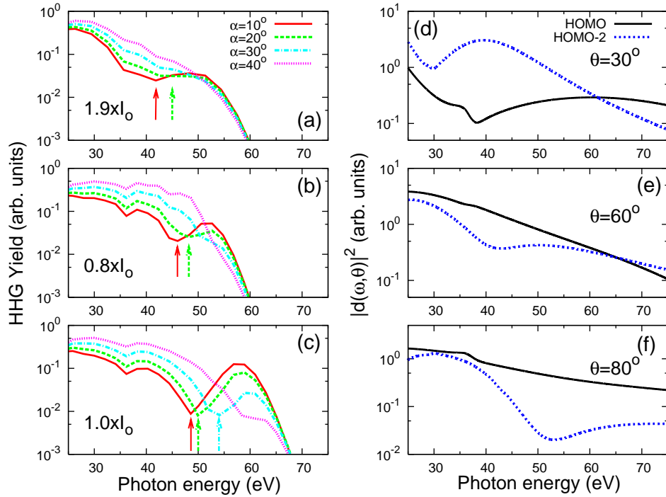
FIG. 7: (Color online) Dependence of macroscopic HHG spectra (envelope only) on pump-probe angles \alpha=10^\circ , 20^\circ , 30^\circ , and 40^\circ (a) for an 800-nm laser, (b) and (c) for a 1200-nm laser. Laser intensities are given in units of I_0=10^{14} W/cm 2 . Arrows indicate the positions of minima. Degree of alignment: \langle \cos^2 \theta \rangle = 0.60 . (d)-(f) Photorecombination transition dipoles (parallel component, the square of magnitude) of HOMO and HOMO-2 in terms of photon energy at alignment angles \theta=30^\circ , 60^\circ , and 80^\circ .
