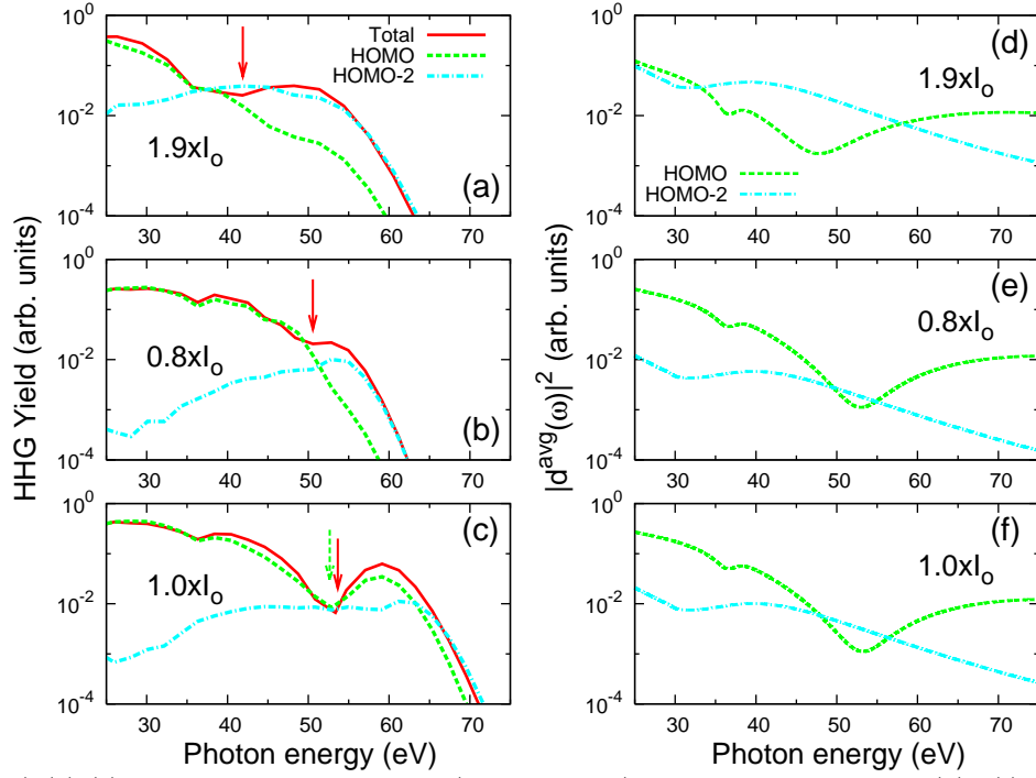
FIG. 2: (Color online) (a)-(c) Macroscopic HHG spectra (envelope only) corresponding to Figs. 1(d)-1(f), respectively. Total (HOMO and HOMO-2 together) spectra and the spectra of individual HOMO and HOMO-2 are shown. (d)-(f) Averaged photorecombination transition dipoles (parallel component, the square of magnitude) of HOMO and HOMO-2 corresponding to (a), (b), and (c), respectively. Laser intensities are indicated where I_0 = 10^{14} W/cm 2 . Arrows indicate the positions of minima. Pump-probe angle \alpha = 0^\circ .
