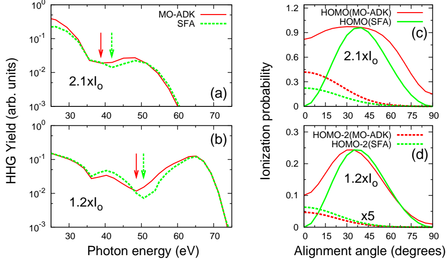
FIG. 5: (Color online) Dependence of macroscopic HHG spectra (envelope only) on the ionization probabilities calculated from MO-ADK or SFA in (a) an 800-nm laser, and (b) a 1200-nm laser. Laser intensities are indicated where I_0=10^{14} W/cm 2 . Arrows indicate the positions of minima. Degree of alignment: \langle \cos^2\theta \rangle = 0.60 . Pump-probe angle \alpha=0^\circ . (c) and (d) Alignment-dependent ionization probabilities of HOMO and HOMO-2 calculated using MO-ADK and SFA. Laser parameters are the same as (a) and (b). Ionization probabilities of HOMO-2 in (d) are multiplied by 5.
