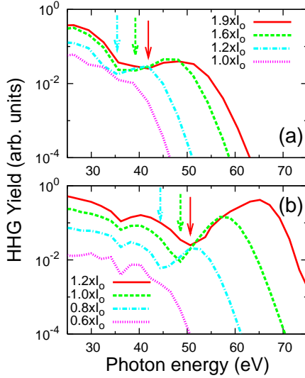
FIG. 3: (Color online) Laser intensity dependence of macroscopic HHG spectra (envelope only) (a) in an 800-nm laser and (b) in a 1200-nm laser. Intensities are shown in units of I_0=10^{14} W/cm 2 . Arrows indicate the positions of minima. Degree of alignment: \langle \cos^2 \theta \rangle = 0.60 . Pump-probe angle \alpha = 0^\circ .
