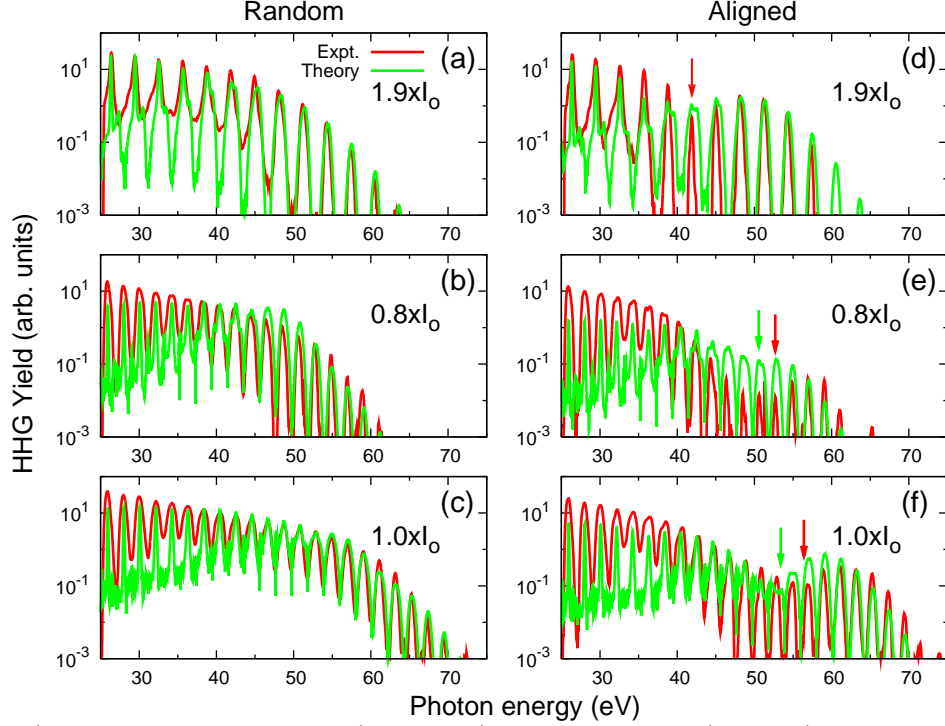
FIG. 1: (Color online) Comparison of theoretical (green lines) and experimental (red lines) HHG spectra of random and aligned \text{CO}_2 molecules, in an 800-nm laser shown in (a) and (d), and in a 1200-nm laser shown in (b), (c), (e), and (f). Laser intensities are indicated where I_0=10^{14} W/cm 2 . Experimental data are from Ref. [49]. Arrows indicate the positions of minima. Pump-probe angle \alpha=0^\circ . See text for additional laser parameters and experimental arrangements.
