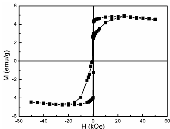
Fig. 5. M-H curve of Mn 3 O 4 nanowires at 5 K.
