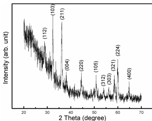
Fig. 2. XRD patterns of \text{Mn}_3\text{O}_4 nanowires.
