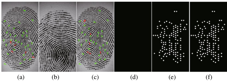
Fig. 13 Tamper detection under collage a fingerprint 1# and its minutiae b fingerprint 2# c tampered fingerprint 1# and its minutiae d detection result by Yeung et al. [22] e detection result by our method f tamper mask
