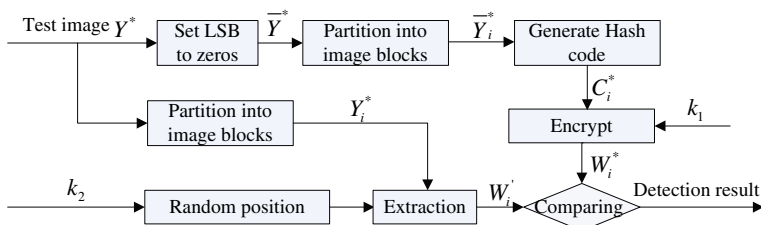
Fig. 5 Flowchart of watermark extraction and tamper detection
