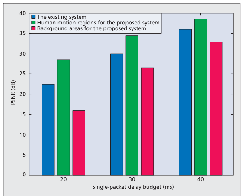
Figure 6. PSNR comparison of different single-packet delay deadlines.
